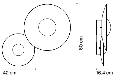
Accessory C2 42/60
