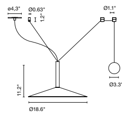
Milana 47 Counterweight
