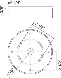
Mounting plate detail:
